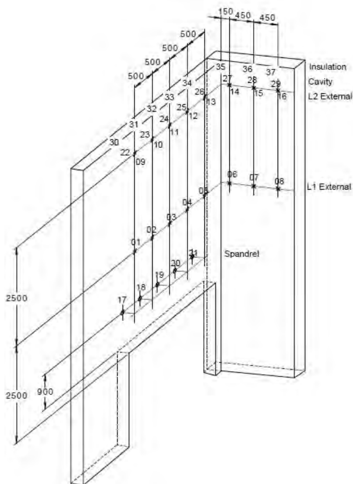
FIGURE 9: THERMOCOUPLE LOCATION
